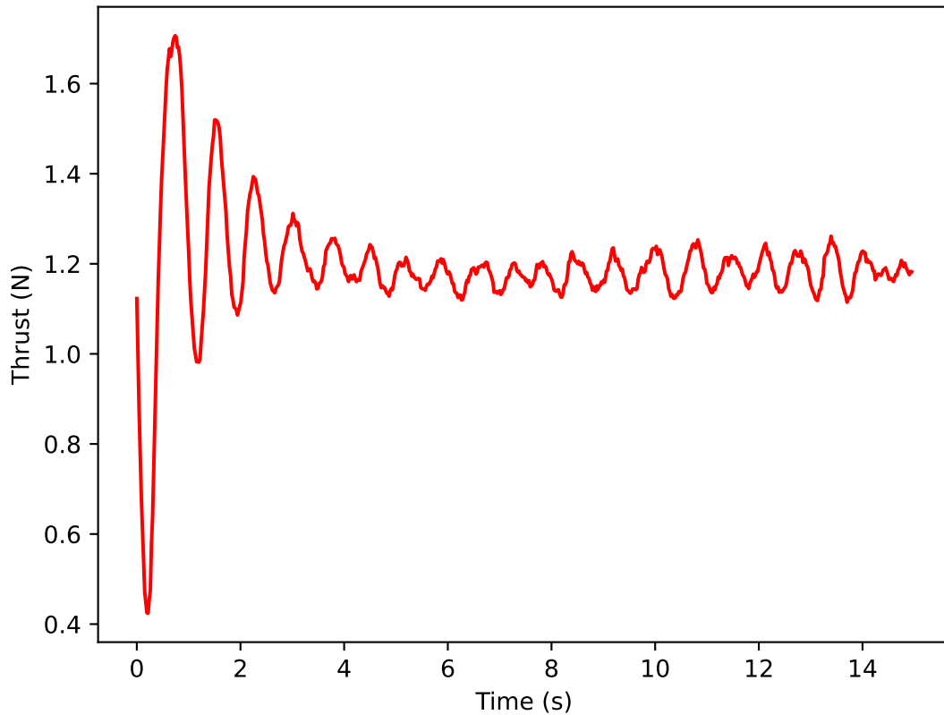
Cruise Thrust Plot
