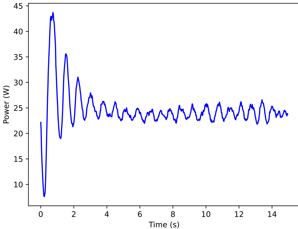
Cruise Power Plot
