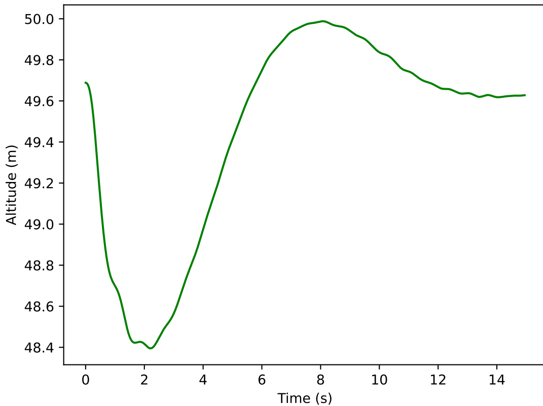
Cruise Altitude Plot
